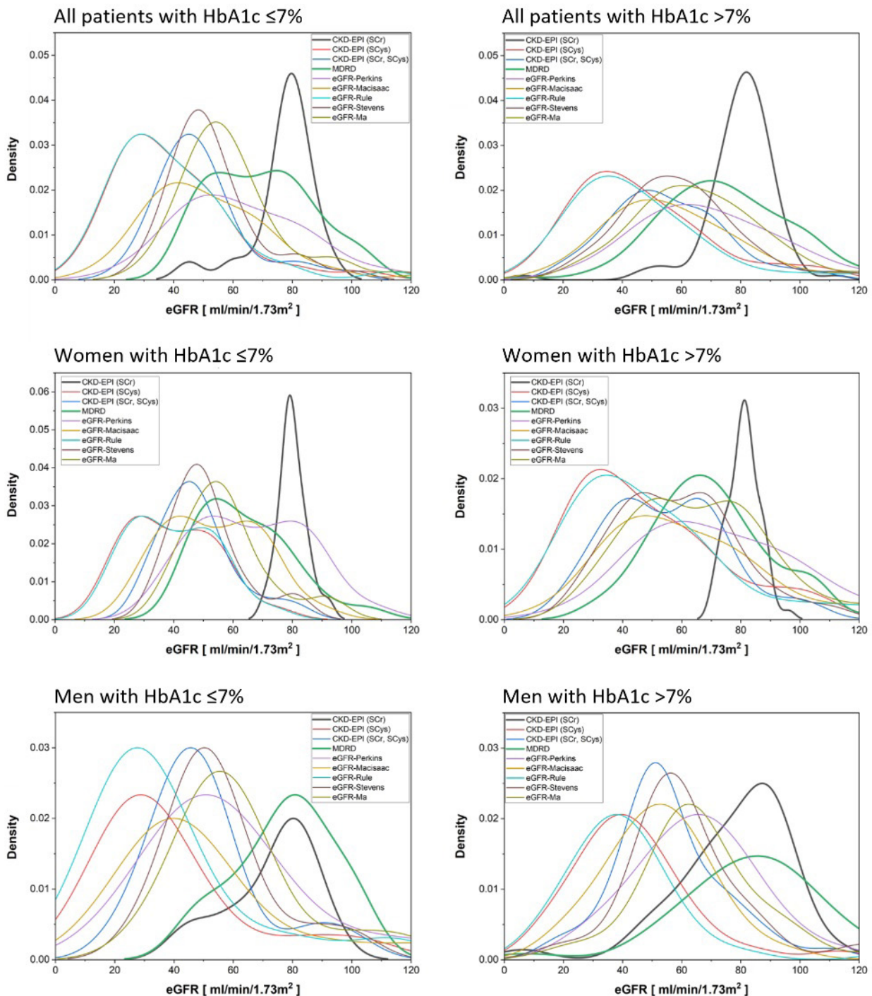
Fig. 1. Distribution of estimated glomerular filtration rate calculated with various eGFR equations demonstrated as a kernel density plot
